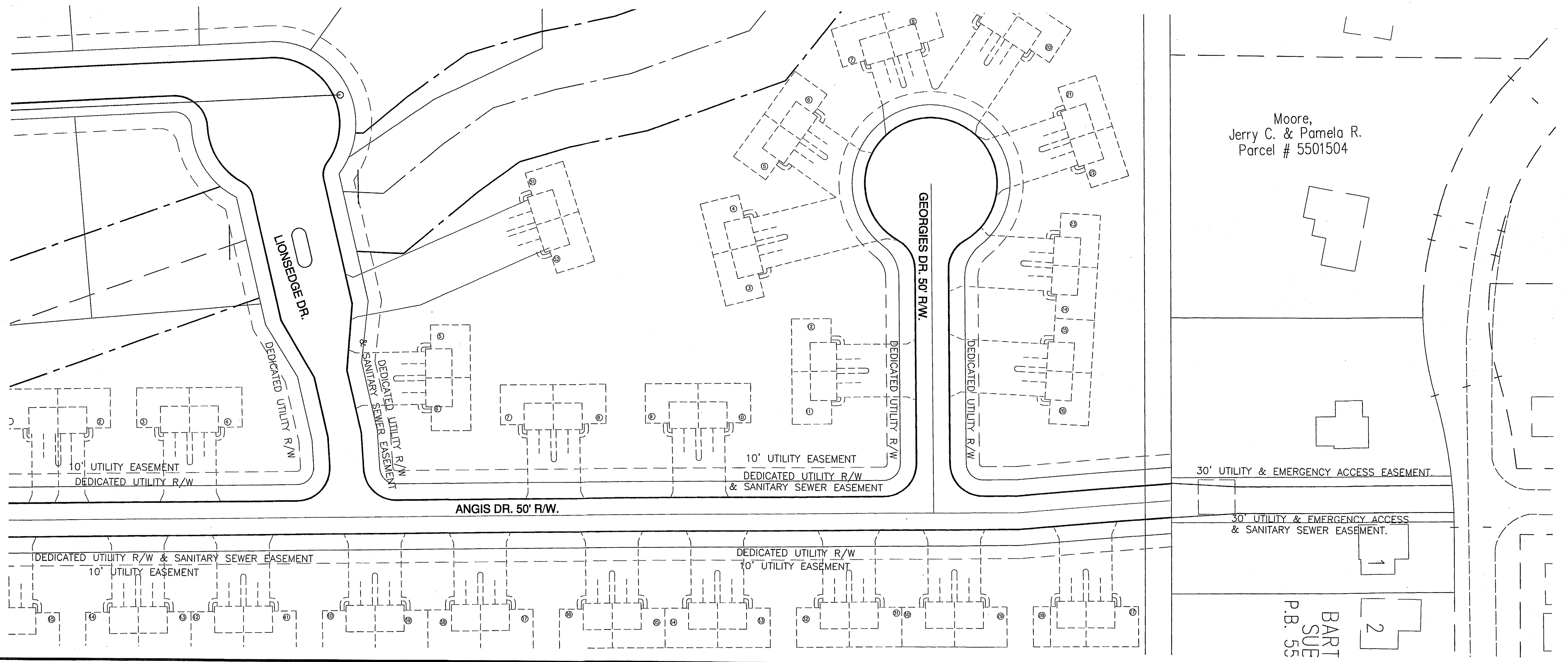
EASEMENT PLAN SCALE = 1" = 40'
