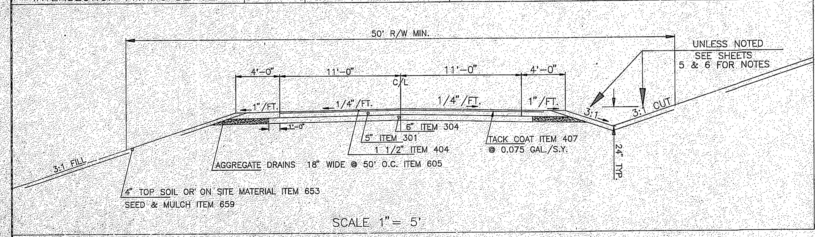
TYPICAL FLEXIBLE PAVEMENT ROADWAY SECTION
