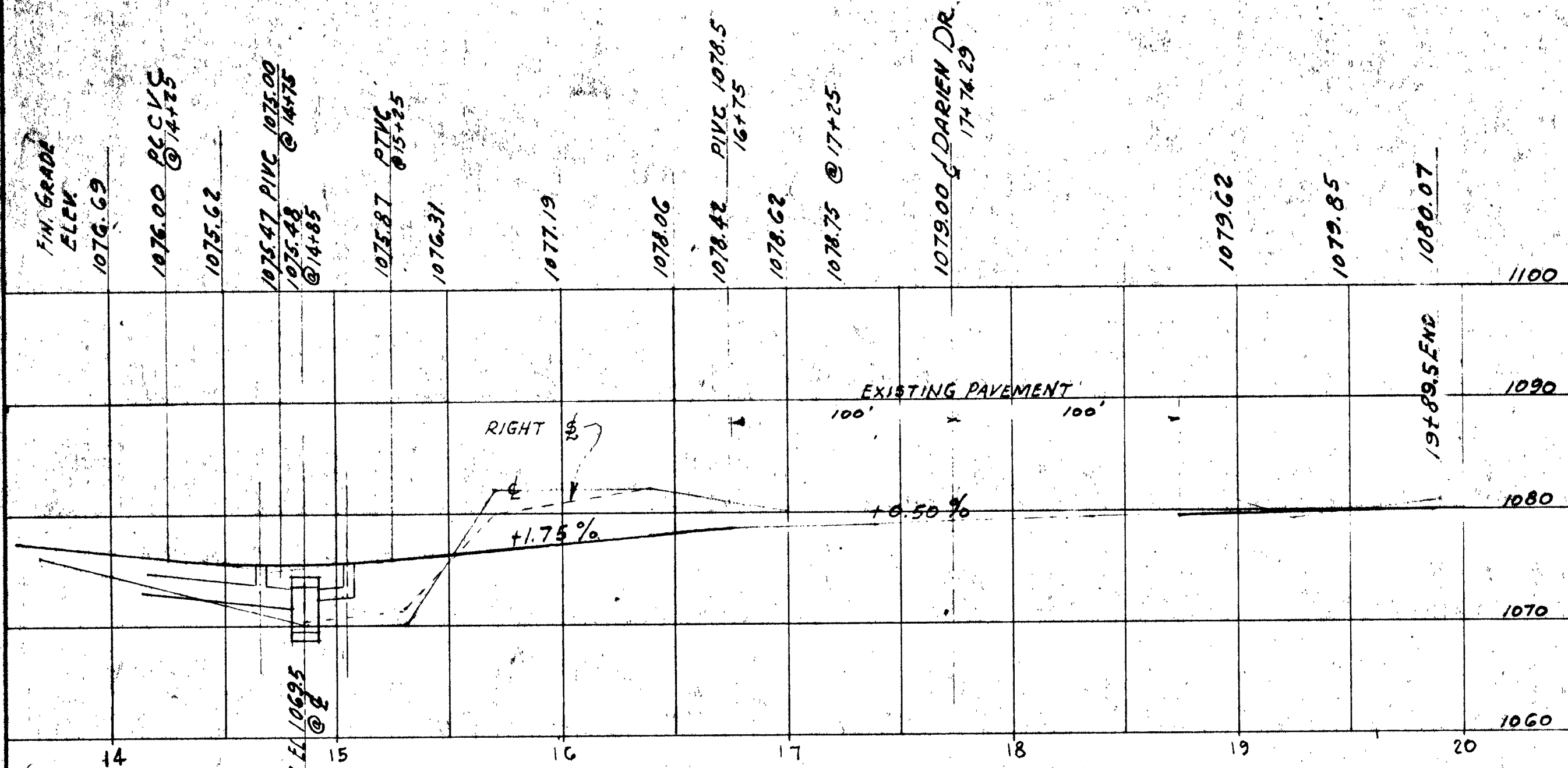
PROFILE SCALE 1" = 50' HORIZ. 1" = 10' VERT.
