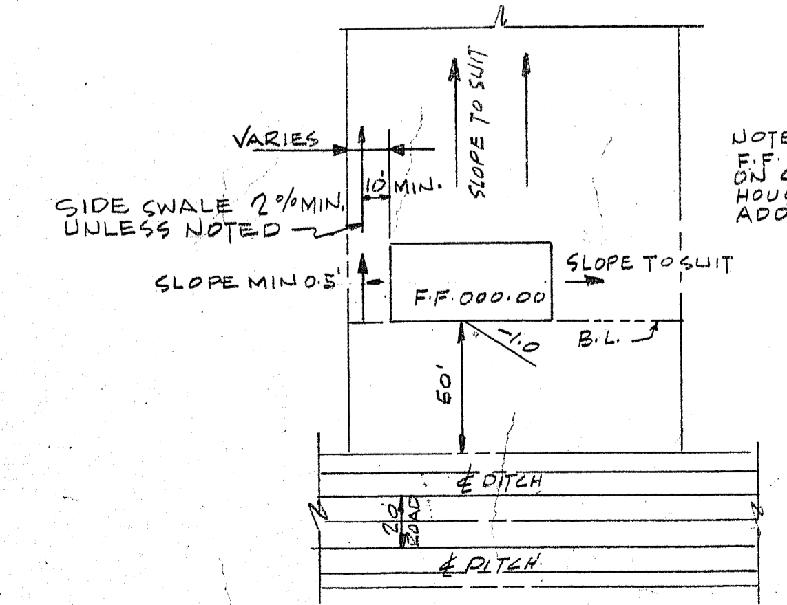
TYPICAL PLAN TYPE "B" GRADING
