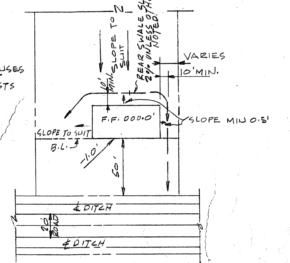
TYPICAL PLAN TYPE "A" GRADING
