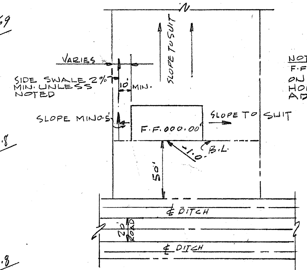
TYPICAL PLAN TYPE 'B' GRADING
