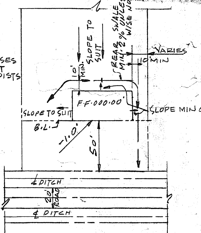
TYPICAL PLAN TYPE 'A' GRADING
